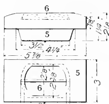
Figs. 5150-5151. Stop-wedge.
